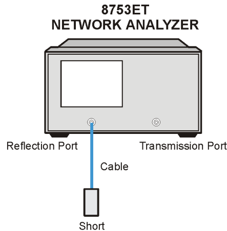
Figure 3-6 Second Connection for Insertion Loss Measurement (8753ET)
