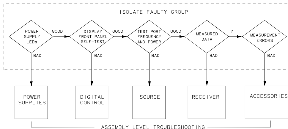
Figure 4-2 Troubleshooting Organization
