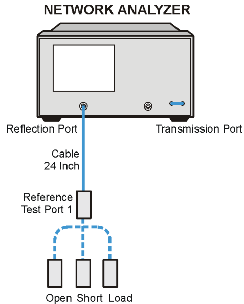
Figure 2-76 Second Enhanced Response Calibration
