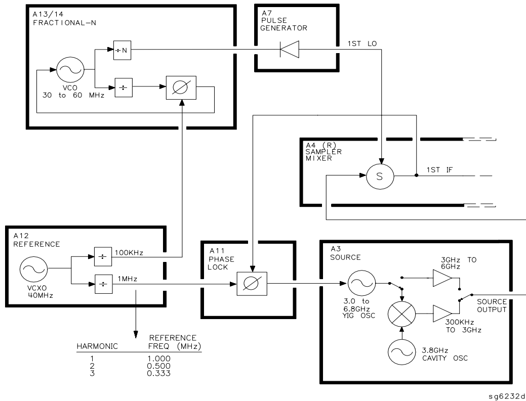
Figure 12-6 Harmonic Analysis
