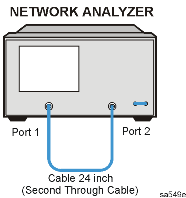
Figure 3-9 Connections for the Second Through Cable
