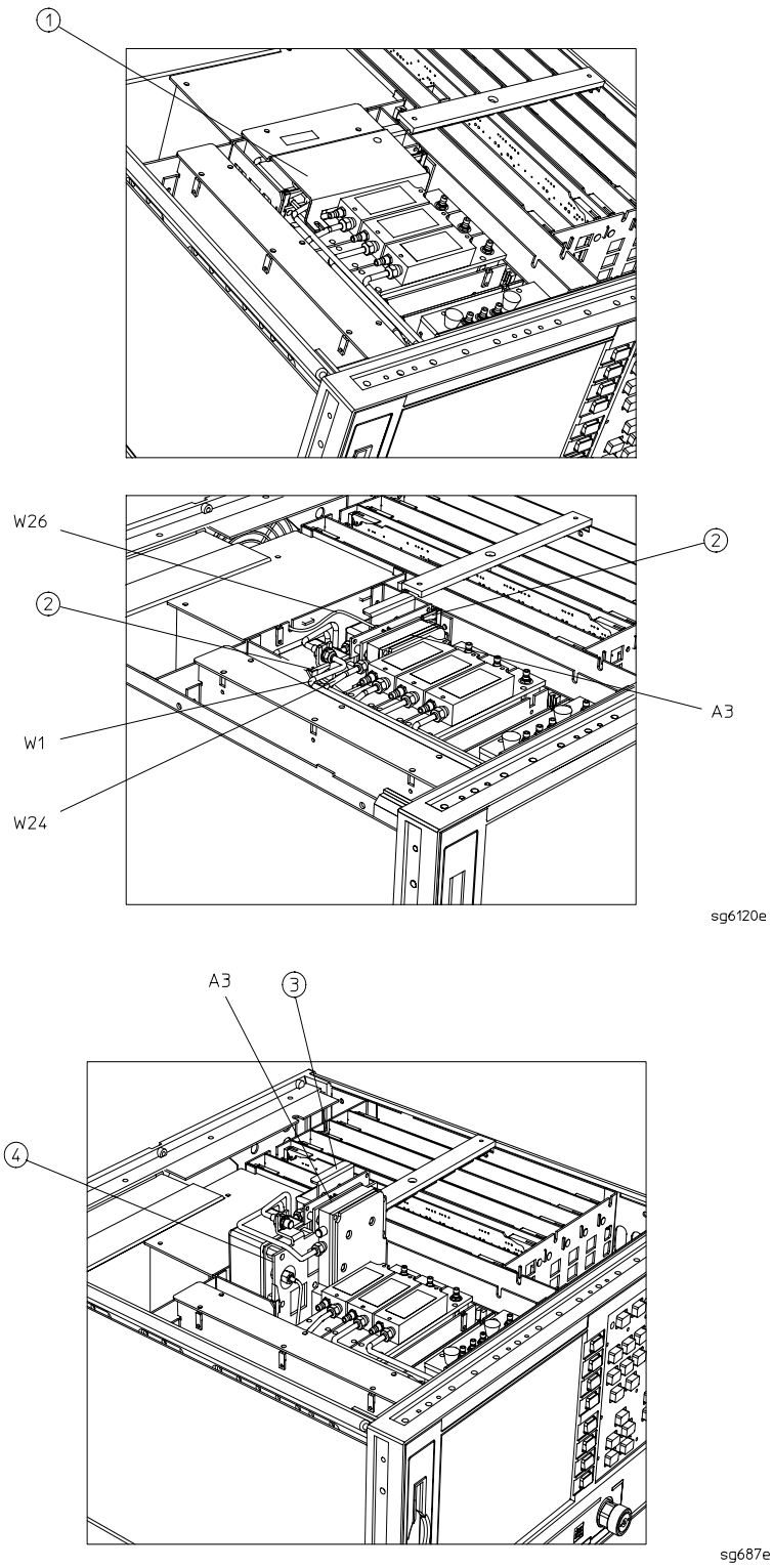
Figure 14-8 A3 Source Assembly
